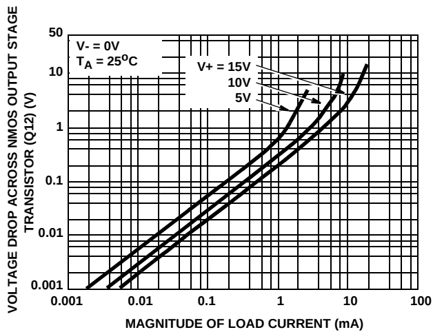
FIGURE 21. VOLTAGE ACROSS NMOS OUTPUT STAGE TRANSISTOR (Q 12 ) vs LOAD CURRENT
