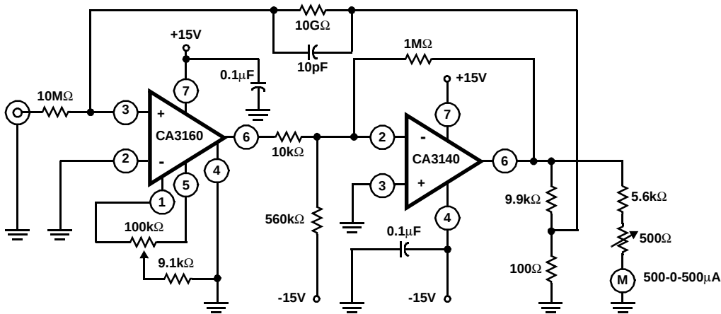
FIGURE 11. CURRENT-TO-VOLTAGE CONVERTER TO PROVIDE A PICOAMMETER WITH \pm 3 pA FULL SCALE DEFLECTION
