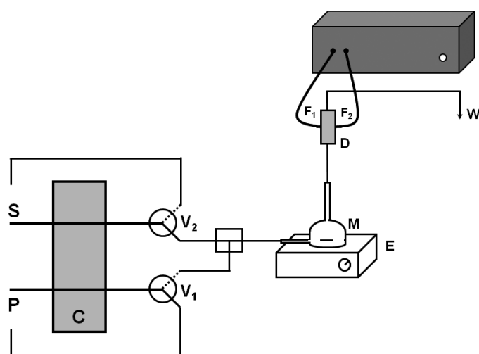
FIG. 2. Flow system scheme for concentration perturbation. (C) peristaltic pump, (S) sample, (P) perturbing substance, (V1) and (V2) solenoid valves for reagents commutation, (M) stirred mixing chamber, (D) detection cell (optic path approximately 5.0 mm), (E) magnetic stirrer, (F1) and (F2) optical fiber bundles, and (W) waste.
