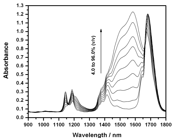
Fig. 3. NIR spectral set obtained for mixtures of ethanol and toluene (4% to 96% v/v).
