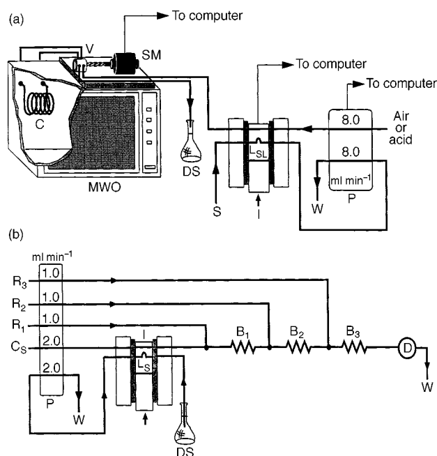
Fig. 1 (a) Flow diagram of the on-line sample digestion system. P, peristaltic pump; W, waste; L SL , slurry sample loop (200 \mu\text{l} ); S, slurry sample; I, injector commutator; DS, digested sample; SM, stepped motor; V, digestion valve; C, digestion coil (2 m long) and MWO, microwave oven; DS, (b) Flow diagram for FI spectrophotometric determination of iron. L S , sample (200 \mu\text{l} ); C S , carrier; R 1 , ascorbic acid; R 2 , 1,10-phenanthroline; R 3 , acetate buffer; B 1 , B 2 and B 3 , mixing coils of 10, 25, and 30 cm, respectively; D, detector (512 nm). Other symbols as Fig. 1(a).
